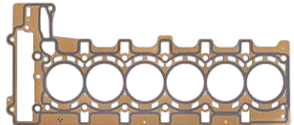
Gasket, cylinder head 1.12mm thickness (4-lyr) # 186.030 # 11 12 7 599 212
