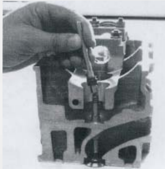
Installation using Elring mounting tool
